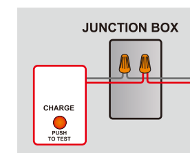
Two-wire illuminated test switch (2w-ITS)
