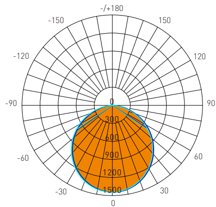
4' / Diffuser / 3500K
