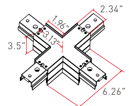
Lit "+" Joiner
