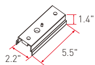
Line Joiner
