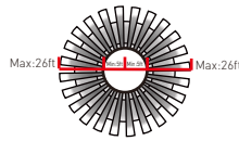
(Height of installation 8ft) Detection Range
